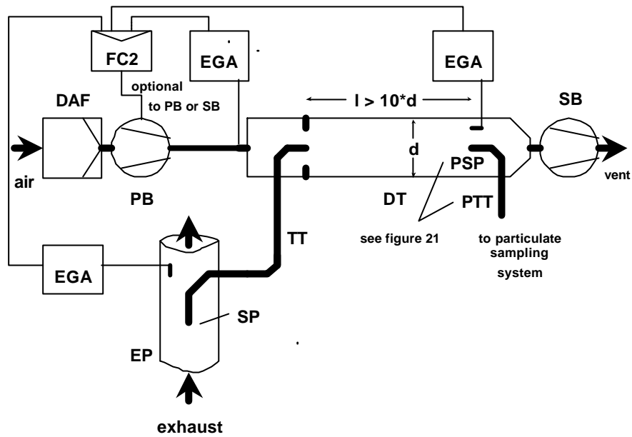
Figure 13 - Partial flow dilution system with \text{CO}_2 or \text{NO}_x concentration measurement and fractional sampling
