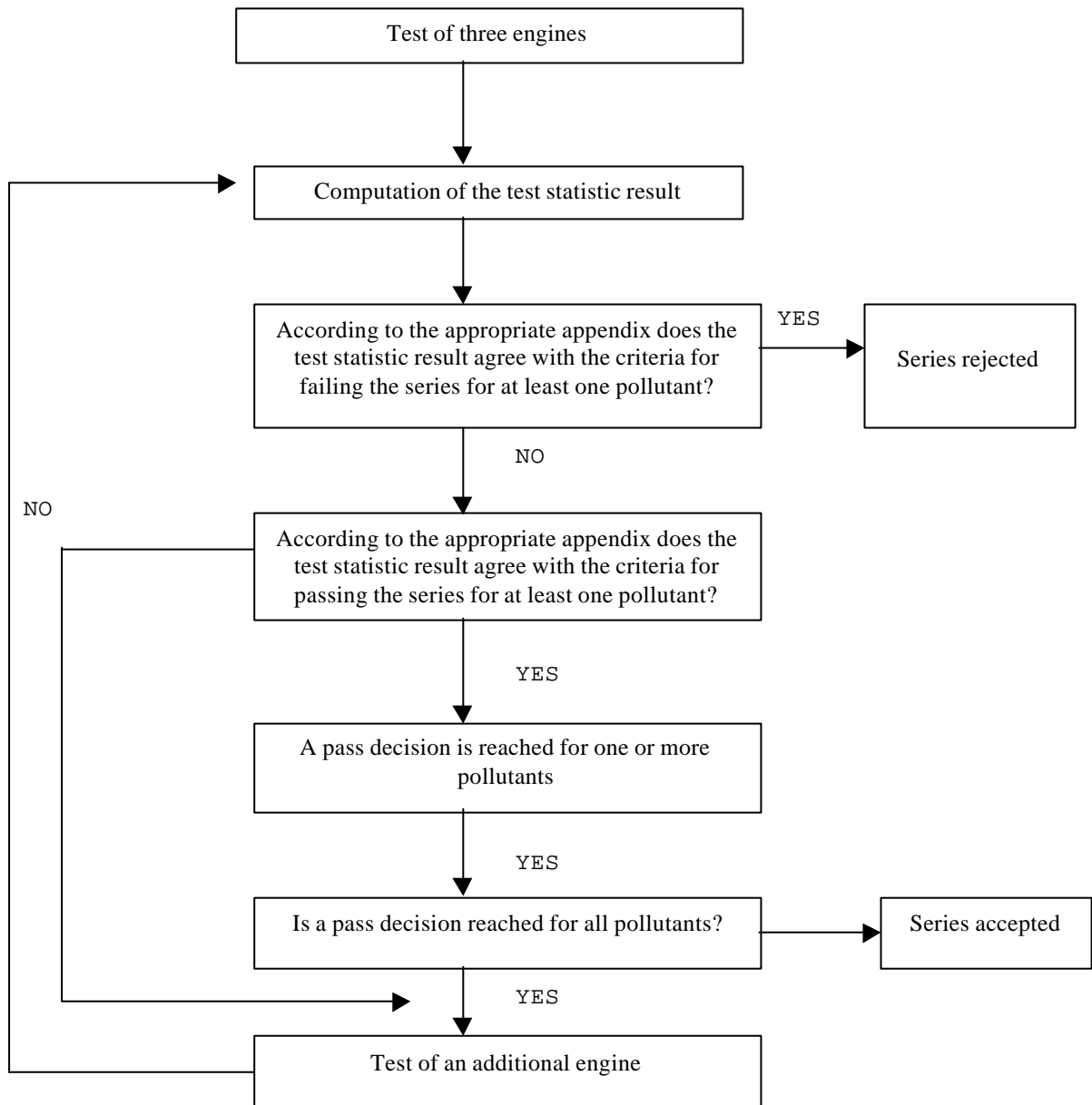
Figure 2: Conformity of production testing scheme"
