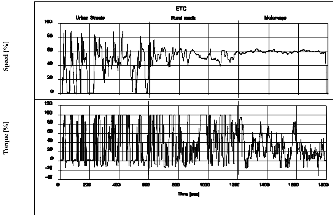
Figure 5: ETC Dynamometer Schedule
