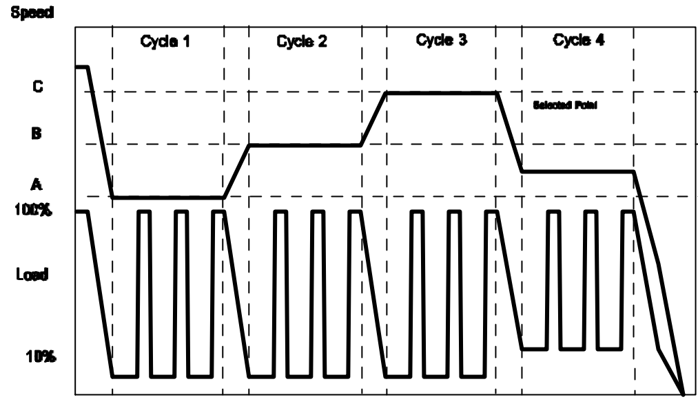
Figure 3: Sequence of ELR Test
