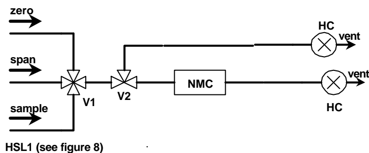
Figure 10 - Flow diagram for methane analysis with the non-methane cutter (NMC)
