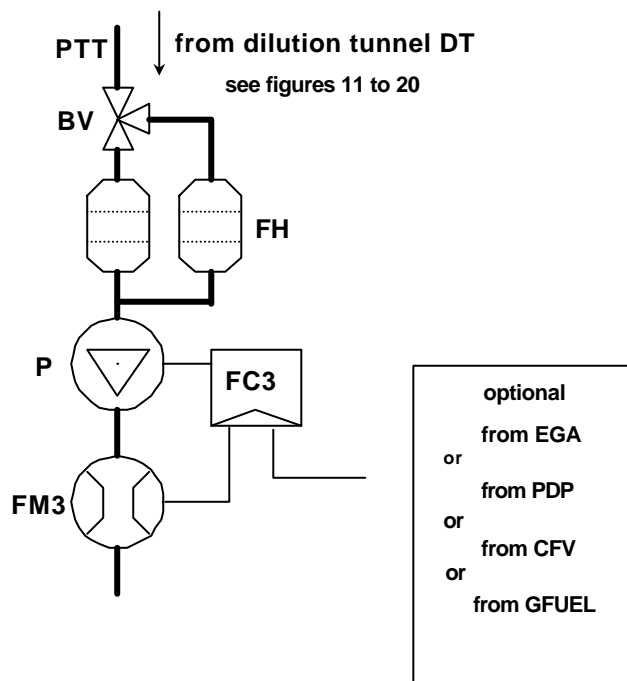
Figure 21 - Particulate sampling system
