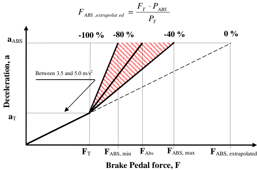
Figure 1a: Pedal force characteristic needed in order to achieve maximum deceleration with category "A" BAS
