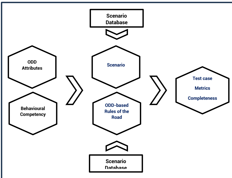
Figure2. Rules of the road as pass/fail criteria.
