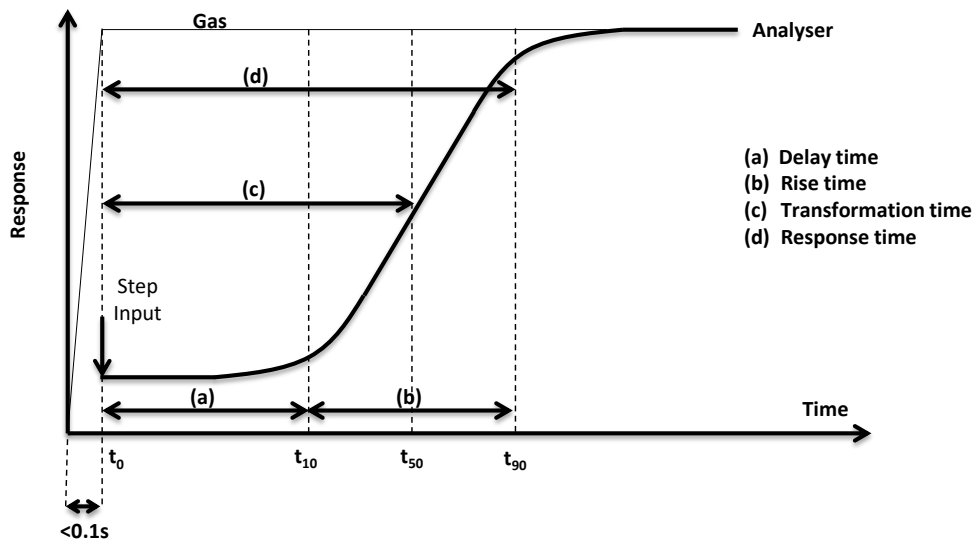
Figure 2 Definition of delay, rise, transformation and response times
