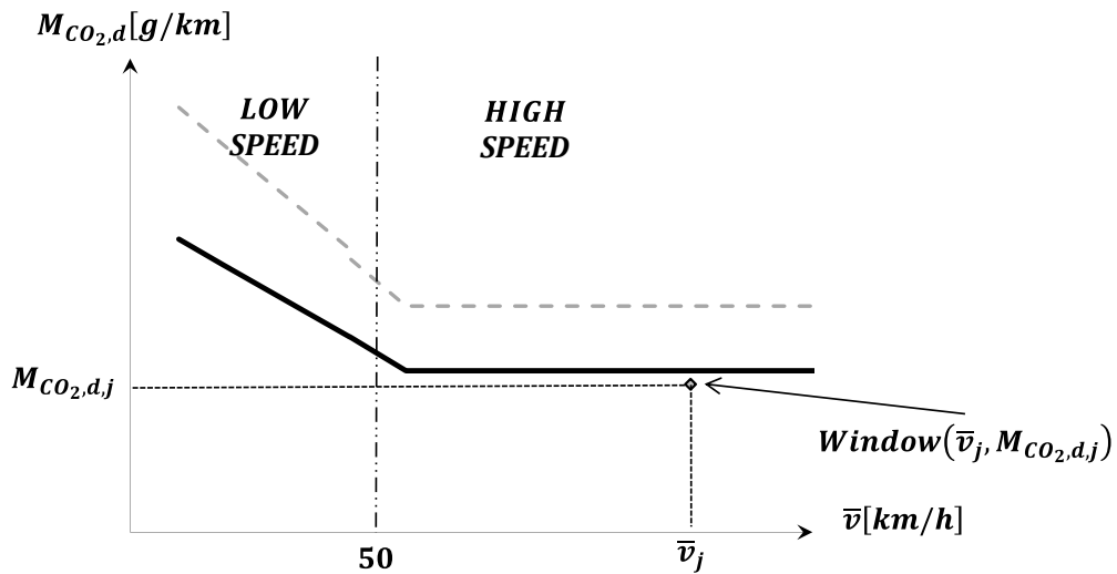
Vehicle CO 2 characteristic curve: low and high speed definitions (Illustrated for OVC-HEV vehicles)
