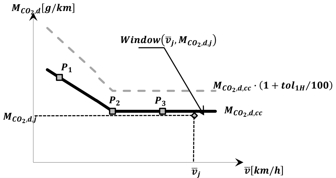
Figure A8/4-2 Vehicle CO 2 characteristic curve and tolerances for OVC-HEV vehicles for 3-phase WLTP
