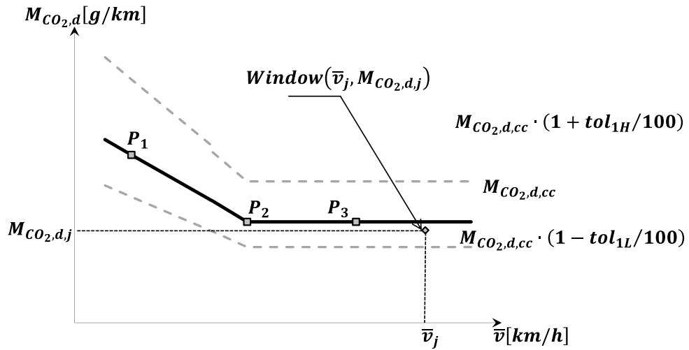
Figure A8/3-2 Vehicle CO 2 characteristic curve and tolerances for ICE and NOVC-HEV vehicles for 3-phase WLTP
