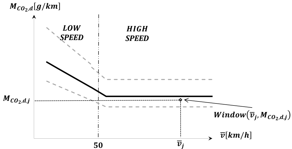
Vehicle CO 2 characteristic curve: low and high speed definitions (Illustrated for ICE and NOVC-HEV vehicles)
