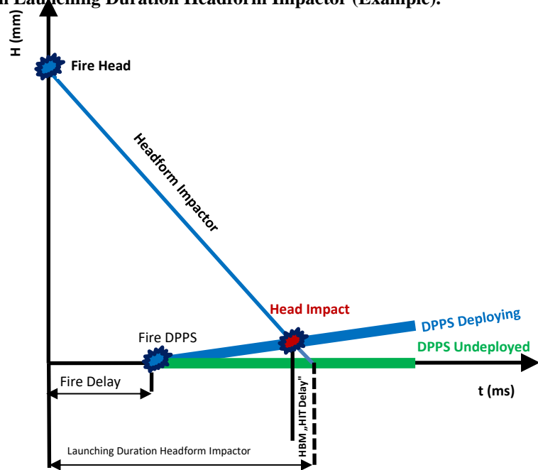
Figure 1 (b) Effect of DPPS Deployment on Launching Duration Headform Impactor (Example).
