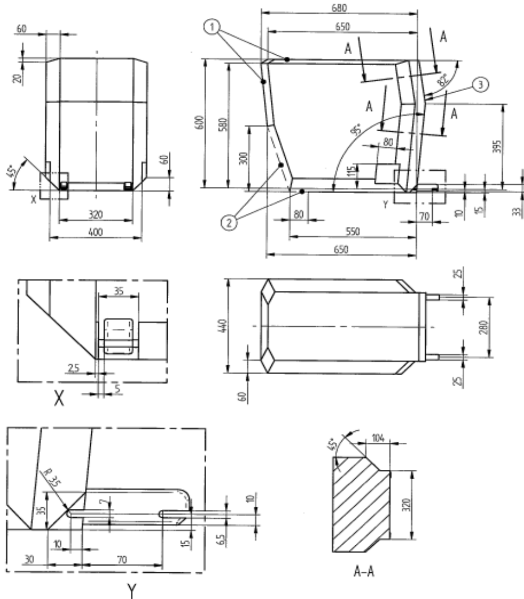
11. Figure 6 ISO/R1 envelope dimensions for an infant-size rearward-facing CRS ISOFIX SIZE CLASS E
