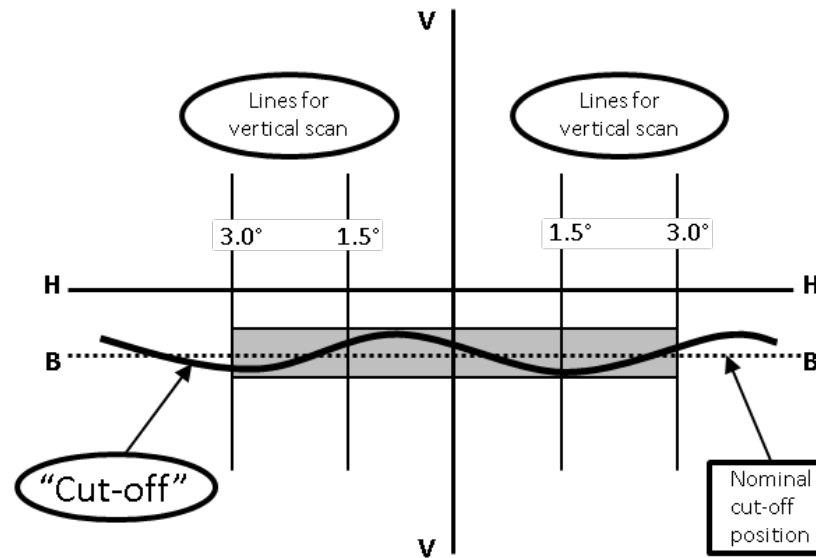
Figure A6-II Measurement of the symmetric "cut-off" quality and instrumental vertical adjustment
