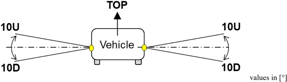
Figure A4-XIII Vertical geometric visibility for cornering lamps
