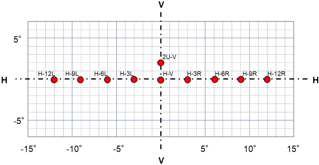
Figure A4-II Driving-beam test points
