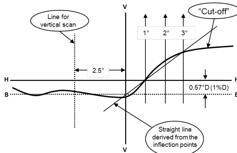
Figure A6-IV Instrumental vertical and horizontal adjustment for asymmetric “cut-off” line - Three-line scan method
