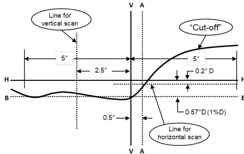
Figure A6-III Instrumental vertical and horizontal adjustment for asymmetric “cut-off” line - horizontal line scan method
