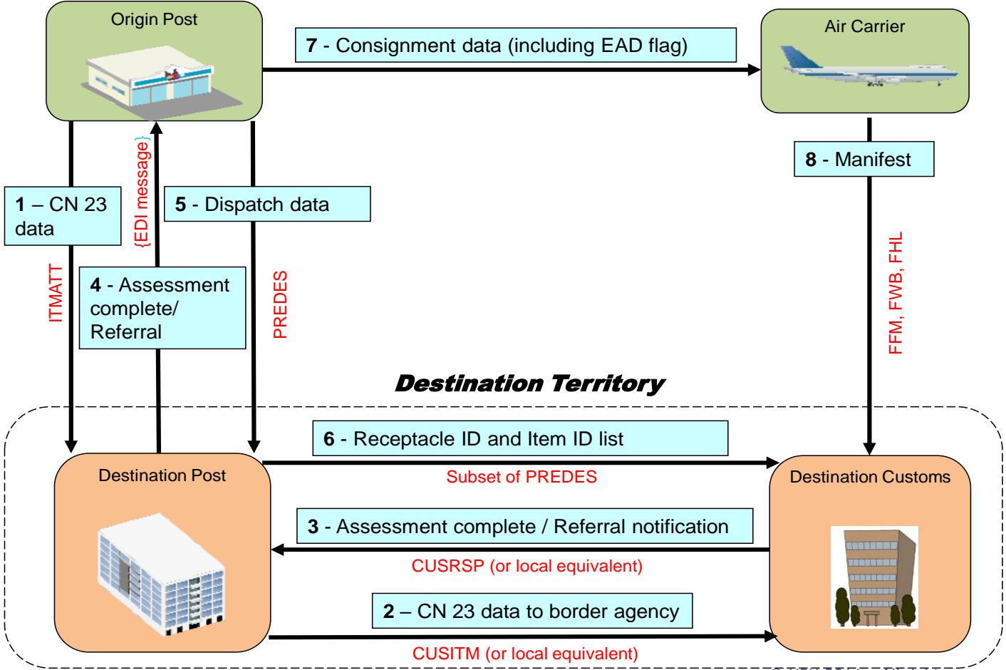
Electronic advance data flowchart (Global Postal Model)
