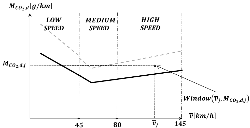
Vehicle CO 2 characteristic curve: low, medium and high speed definitions (Illustrated for OVC-HEV vehicles)
