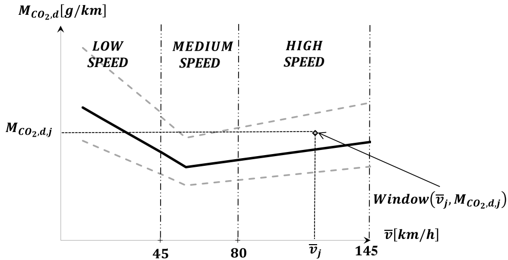
Vehicle CO 2 characteristic curve: low, medium and high speed definitions (Illustrated for ICE and NOVC-HEV vehicles)
