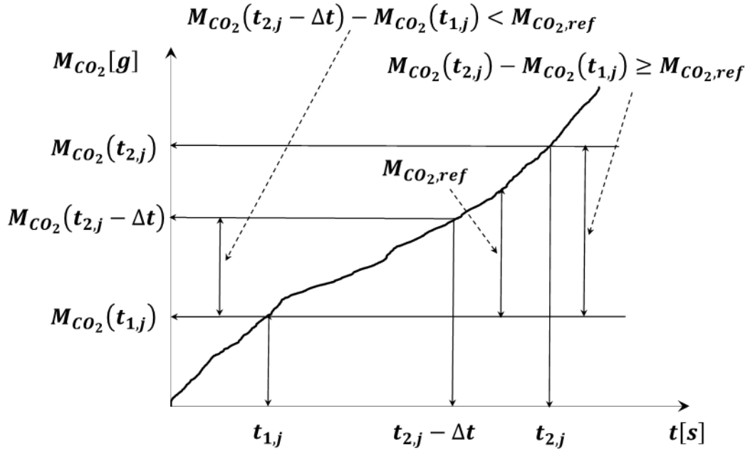
Figure A8/2 Definition of CO 2 mass based on averaging windows
