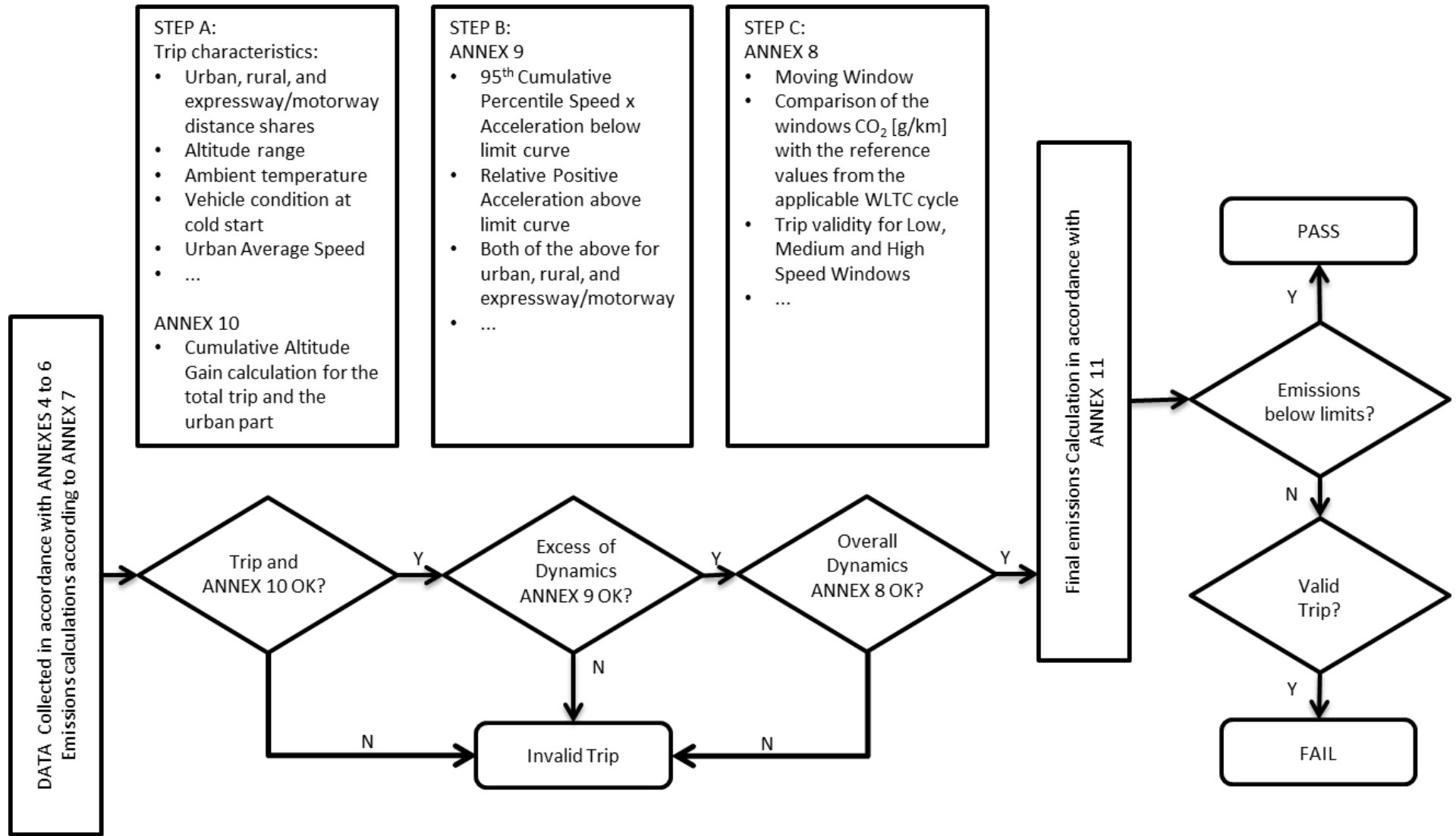
Figure 6 Assessment of trip validity – schematic (i.e. not all details are included in the steps included in the figure, see the relevant annexes for such details)
