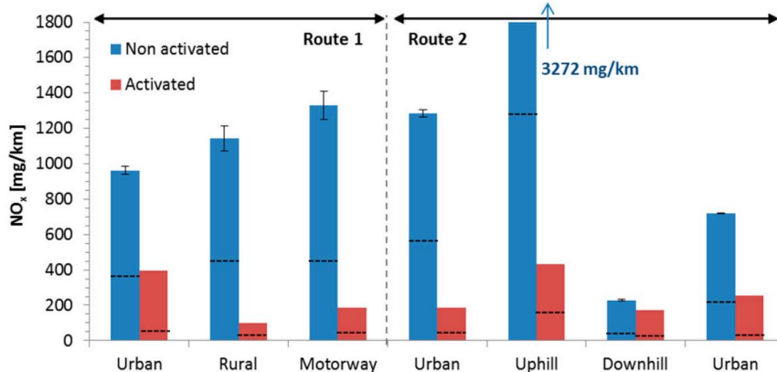
Figure 12: NOx emissions during the real driving emissions testing. Error bars show the maximum and minimum value of the 2 repetitions when available. Dashed lines show the NO 2 emissions. Note that the y axis is cut at 1800 mg/km and the “Uphill” emissions exceeded 3250 mg/km.
