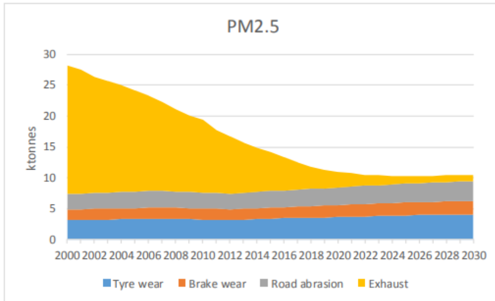
Figure 14: Projected PM 2.5 emissions from road transport for UK [52]
