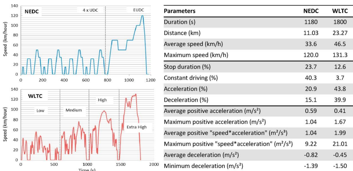
Figure 1: Speed profile and key parameters of the driving cycles NEDC and WLTC (Marotta et al. 2015 [5])
