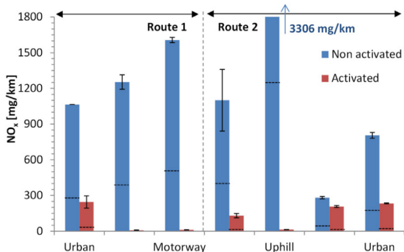
Figure 11: NOx emissions during the real driving emissions testing. The first Urban part is with engine cold start. Error bars show the maximum and minimum value of the 2 repetitions. Dashed lines show the NO 2 emissions (lower part of bars). Note that the y axis is cut at 1800 mg/km and the “Uphill” emissions exceeded 3300 mg/km (Giechaskiel et al., 2018 - [42])
