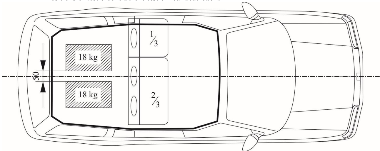
Positions of test blocks before test of rear seat-backs
