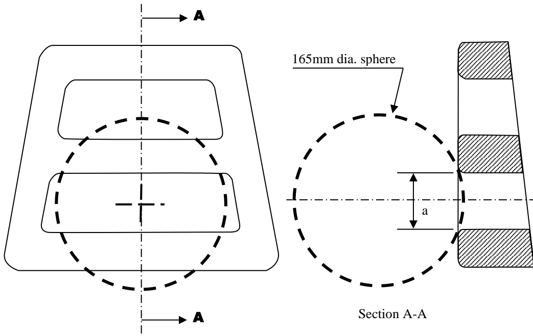
Figure 8-1 Measurement of a Vertical Gap "a"
