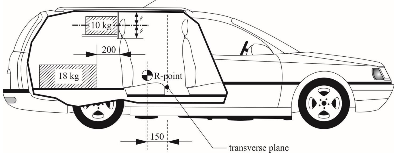
Figure 2 Testing of a partitioning system above the backrest edge of interior roof
