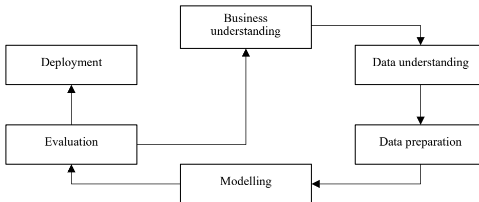
Figure CRISP-DM framework
