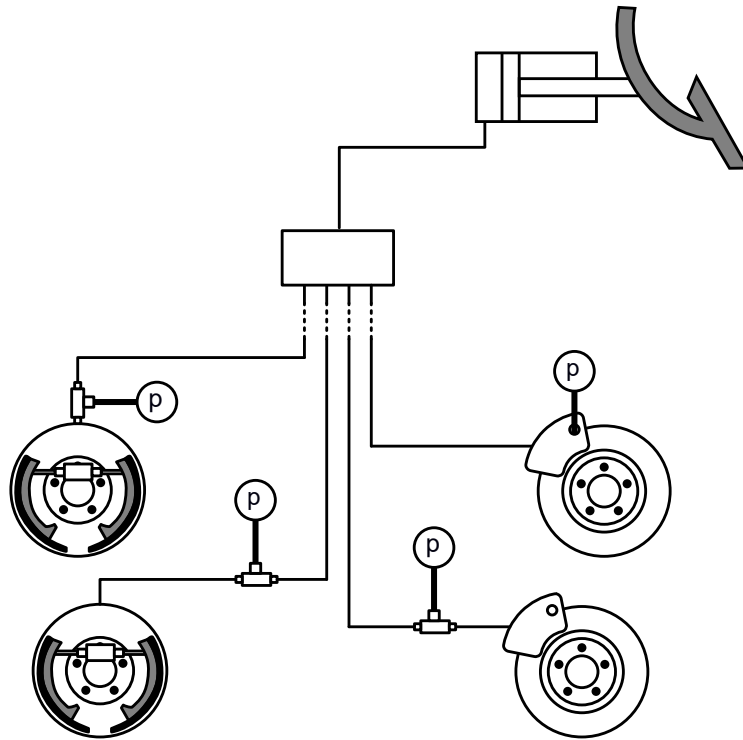
Figure C.4. Examples of mounting of brake pressure sensors (P) at brake pipes of the tested vehicles.
