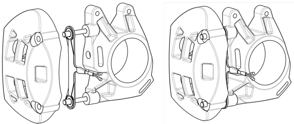
Figure C.1. Schematic example of brake torque sensor mounting.
