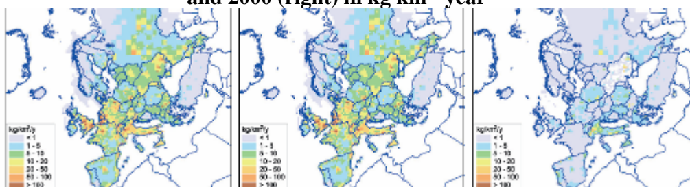
Figure 15: Atmospheric emissions of lead in Europe in 1980 (left), 1990 (middle) and 2000 (right) in \text{kg km}^{-2} \text{year}^{-1}
