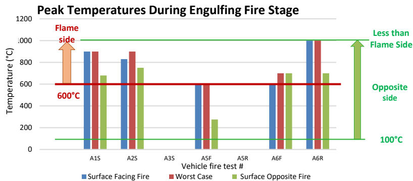
Figure 12 Cylinder temperatures during engulfing fire stage of vehicle fire tests
