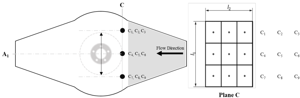
Figure 7.4. Reference positions for airspeed verification
