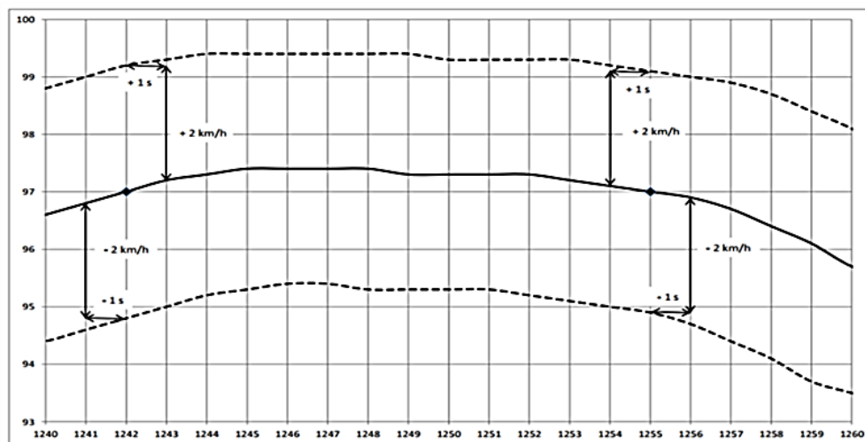
Figure 9.2. Tolerance limits for speed violations during the WLTP-Brake cycle
