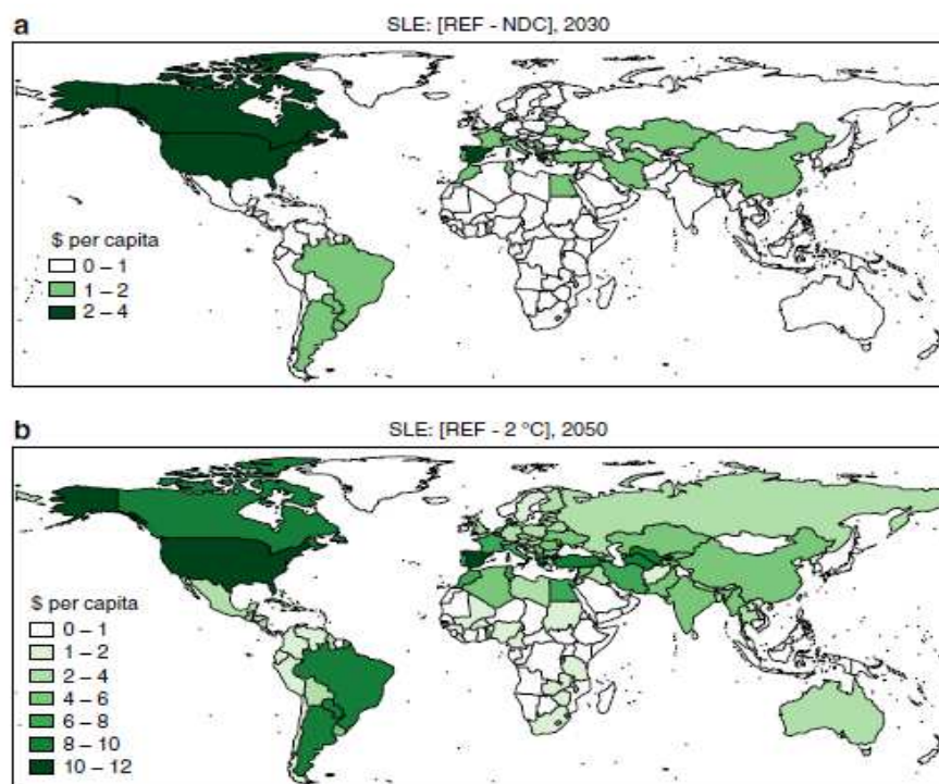
Figure 21 Ozone-related crop yields co-benefits from climate policies, copied from Vandyck et al., 2018 46 . Upper panel – difference between reference scenario and Nationally Determined Contributions in 2030; lower panel – difference between reference scenario and 2°C reduction scenario in 2050.
