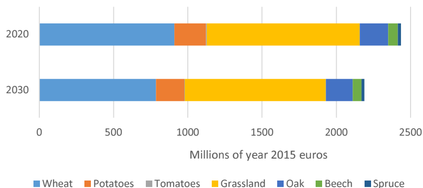
Figure 6 Economic losses from air pollution effects on crops and vegetables in France 22
