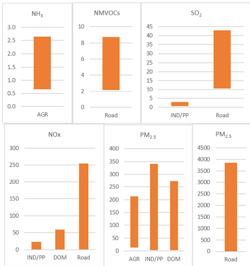
Figure 8 Sector-specific damage cost ranges from air pollutants in Western and Central Europe, thousands year 2015 euros/ton 19,25,26,27,28
