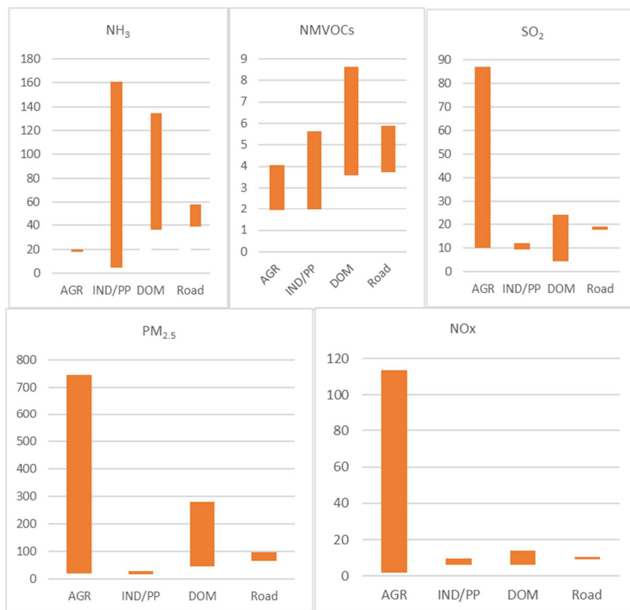
Figure 13 Sector-specific damage costs from air pollutants in the United States of America, thousands year 2015 euros/ton (sources – Goodkind et al., 2019 30 , Schrader et al., 2018 35 ).
