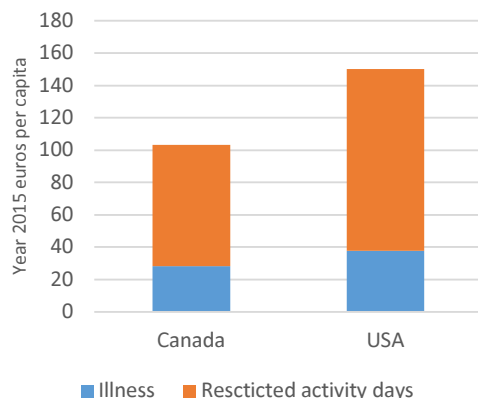
Figure 10 Costs of morbidity in the United States of America and Canada in 2060, based on OECD, 2016 1 .
