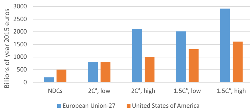
Figure 20 Cumulative health co-benefits (Value of Statistical Life) from climate policies 2020–2050, based on Markandya et al., 2018 45
