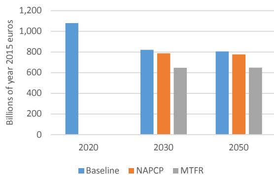
Figure 18 Avoided damage in the European Union-27 due to additional measures beyond the baseline scenario (source - Amann et al., 2020) 5
