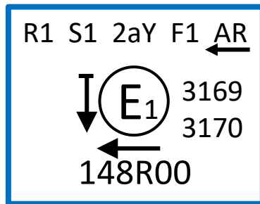
Approval marking
