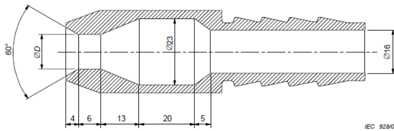
Figure 1 Standard Nozzle for the Test
