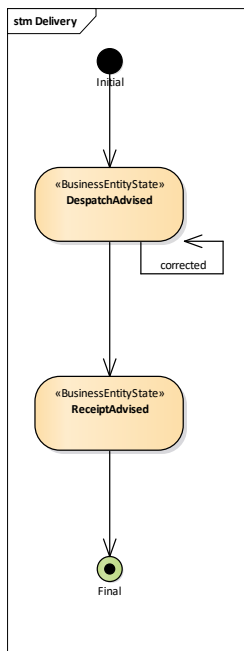
Figure 6-4 Entity Life Cycle diagram
