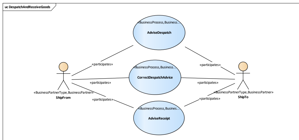
Figure 6-2 Scope of the despatch and receive process
