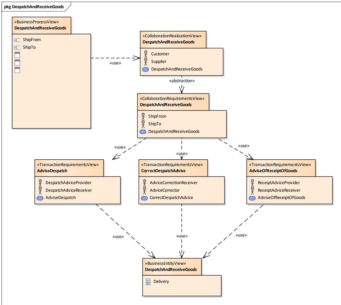
Figure 7-1 Business Information View Despatch And Receipt Of Goods
