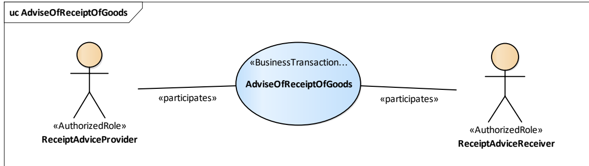
Figure 7-6 Business Transaction Use Case Diagram Advise Receipt
