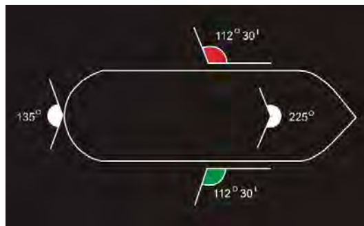
Article 3.01, paragraph 1: The horizontal arc along which the masthead light, the side lights and the stern light are visible.
