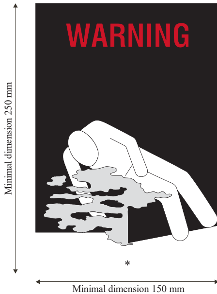
Figure 5.5.2: Asphyxiation warning mark for cargo transport units
