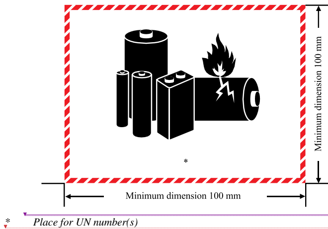
Figure 5.2.5: Lithium battery mark
