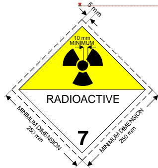
Figure 5.3.1: Placard for radioactive material of Class 7
