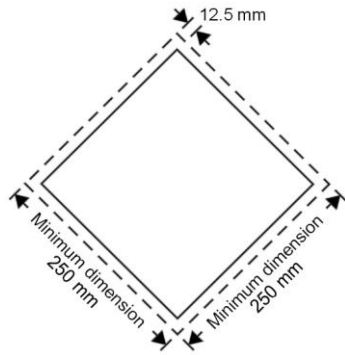
Figure 5.3.0: Placard (except for class 7)
