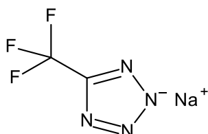
Figure 1: 5-Trifluoromethyltetrazole, sodium salt (TFMT-Na)
