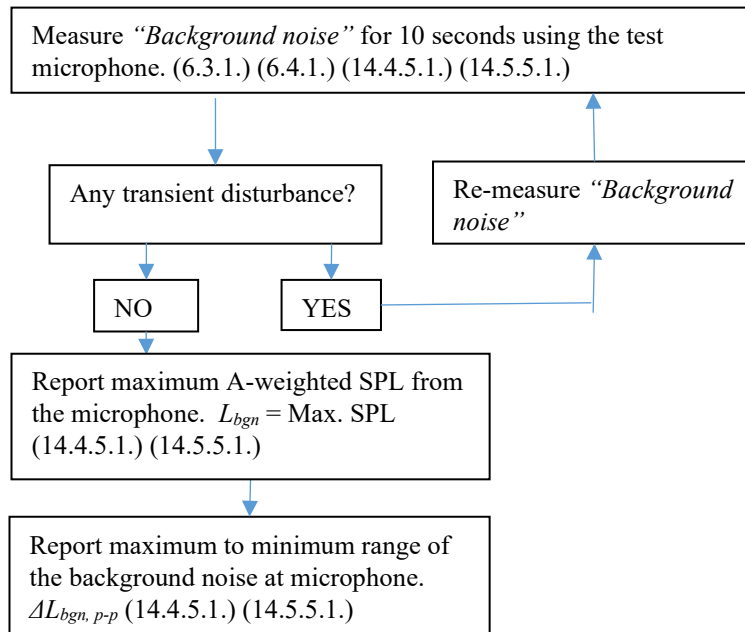
Figure 1 Determination of the range of “Background noise” (14.4.5.) (14.5.5.)
