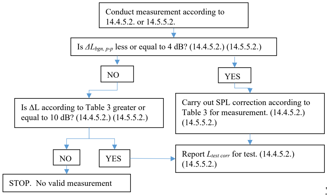
Figure 2 Vehicle A-weighted sound pressure level measurement correction criteria
