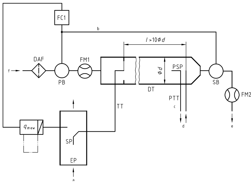
Figure 13 Scheme of partial flow dilution system (fractional sampling type)
