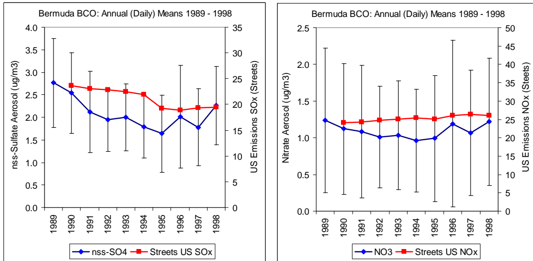
Figure 3.24 Annual mean nss-sulphate and nitrate concentrations on Bermuda during onshore winds compared to the eastern United States \text{SO}_2 ( \text{Tg S}/\text{yr} ) and \text{NO}_x emissions ( \text{Tg N}/\text{yr} ). (Based on data discussed in part in Savoie et al. (2002))
