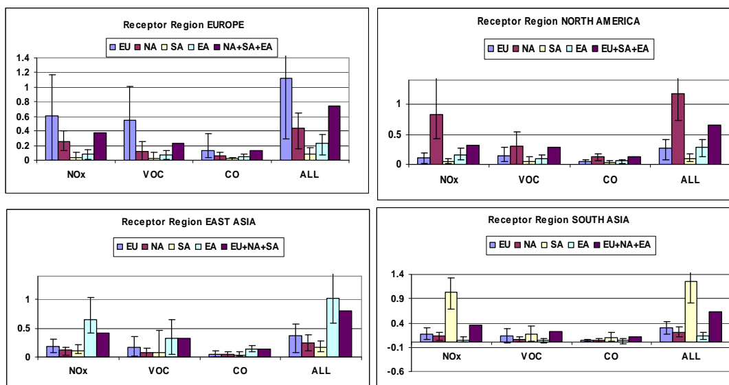
Figure 5.6 Multi-model mean impact of 20 per cent reductions of the ozone precursor emissions (NO x , NMVOCs, and CO) on mean surface ozone over the receptor regions. Decrease in springtime (March-April-May) mean surface O 3 (ppbv) in the HTAP receptor regions resulting from 20 per cent emission reductions of O 3 precursors NO x , NMVOCs, and CO individually within the source regions, and applying all perturbations together (ALL category). Each group of five bars includes the four perturbation experiments; the fifth bar is the sum of the three “foreign” impacts. The bars denote the multimodel mean response (coloured by source region) and the whiskers span the full range of the individual model responses. Results were submitted from 9–14 models for the sensitivity simulations included here.
