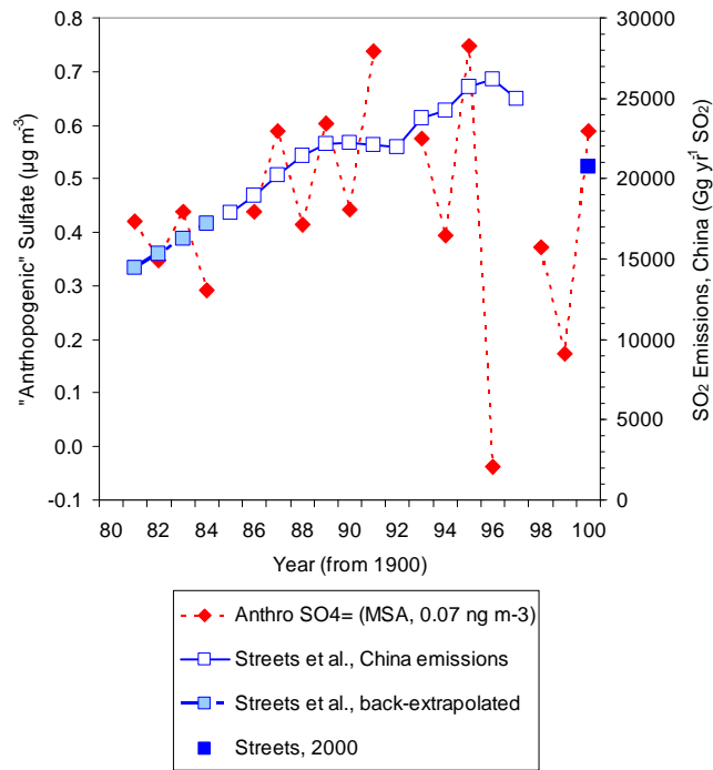
Figure 3.23 Anthropogenic sulphate concentrations on Midway Island compared to the emissions of \text{SO}_2 from China (Prospero et al., 2003).
