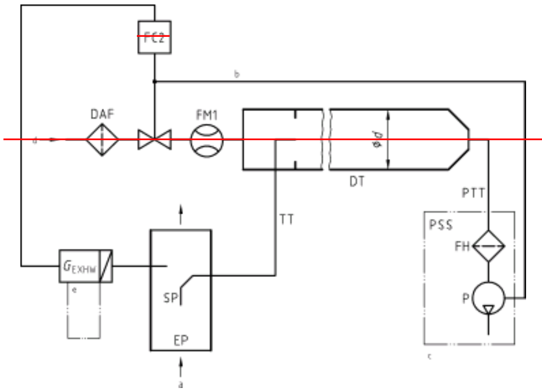
Scheme of partial flow dilution system (total sampling type)
