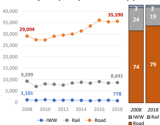
Tonne-km by mode (million) and modal share (%)
