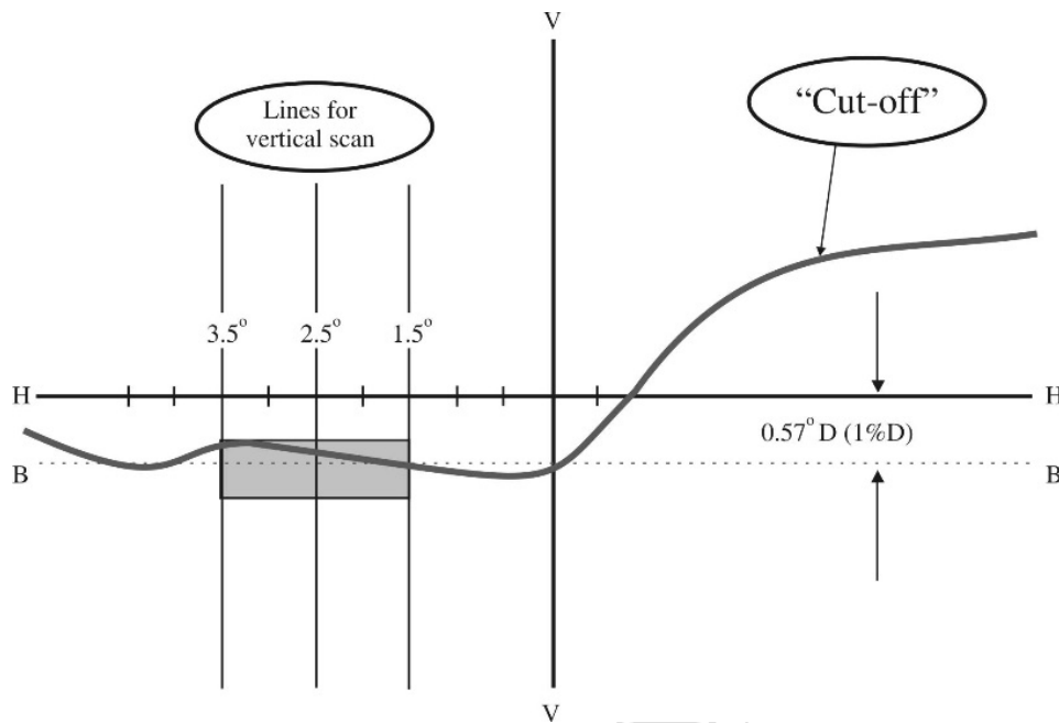
Figure A6-I Measurement of the asymmetric "cut-off" quality
