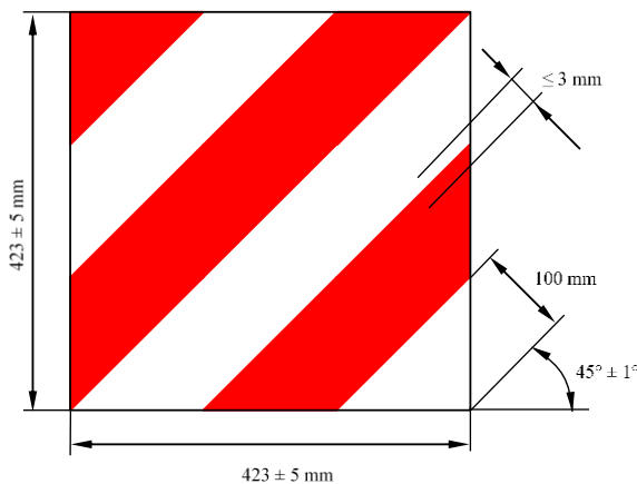
Signalling panel or signalling foil (Form A is shown as an example)
