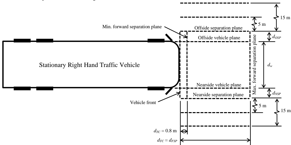
Figure 1 Set Up for Static Crossing Tests
