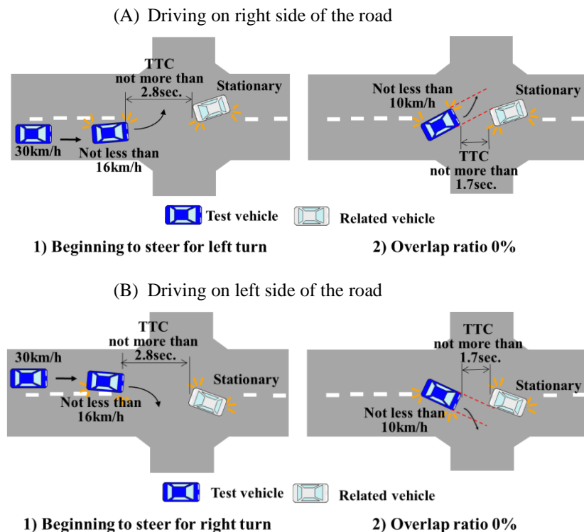
Figure 1 Left turn or right turn at the intersection
