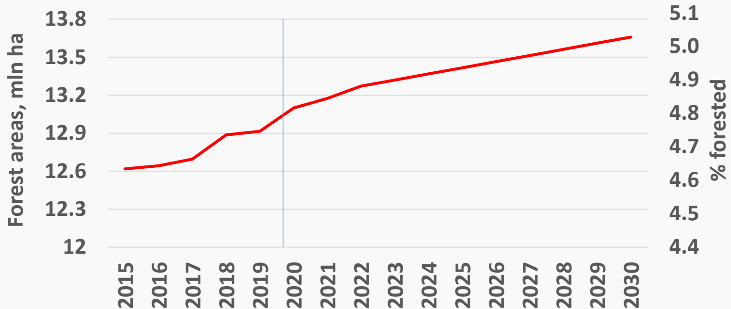
Current forest cover dynamics and future projection
