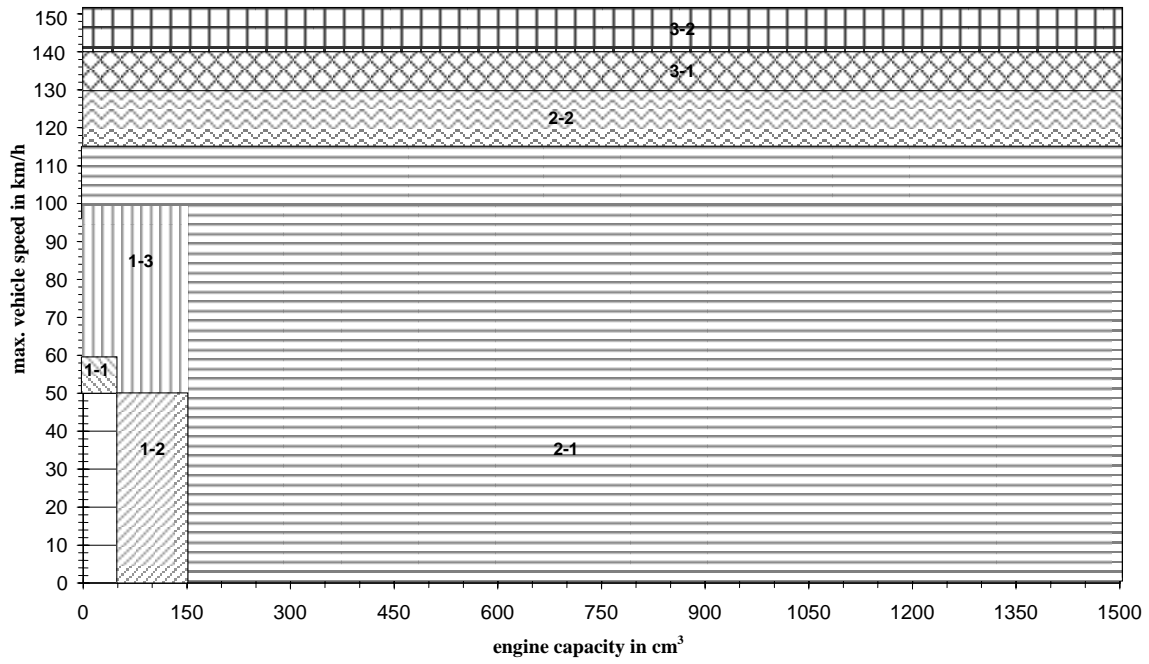
Figure 6-1: vehicle classification
