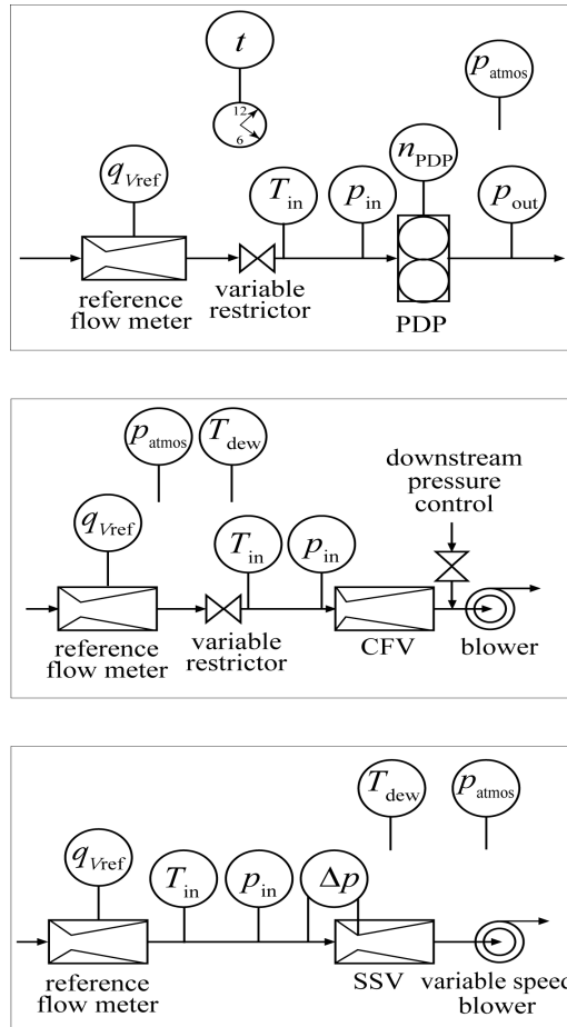
"Figure 8.1 Schematic diagrams for diluted exhaust flow CVS calibration
