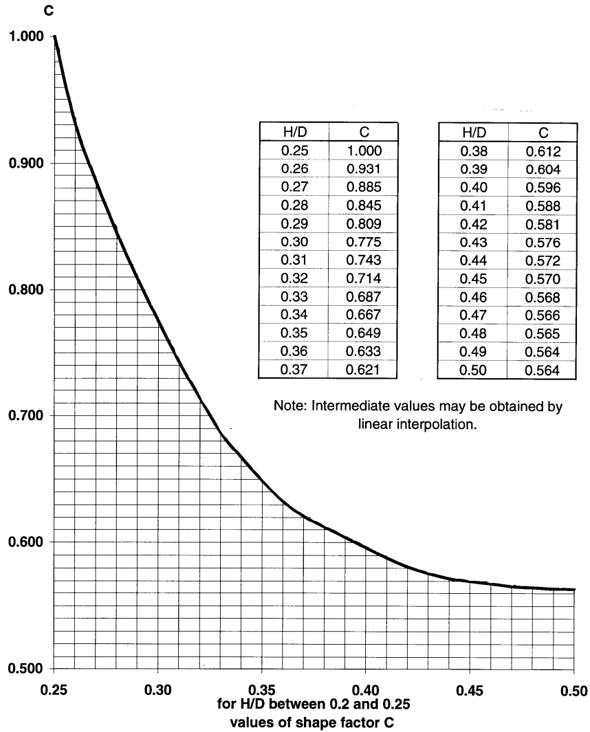
Relationship between H/D and Design factor C
