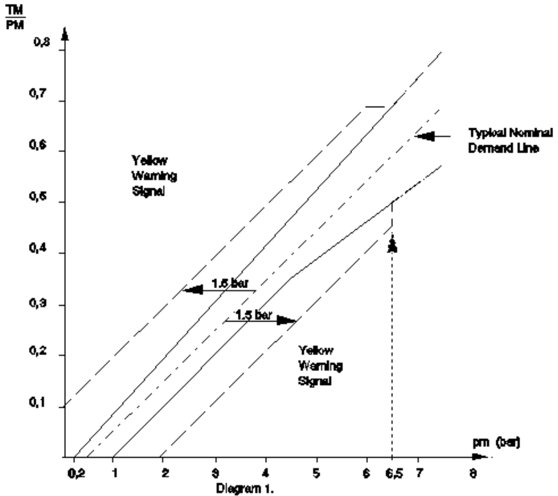
Towing Vehicles for Trailers (except semi-trailers)
