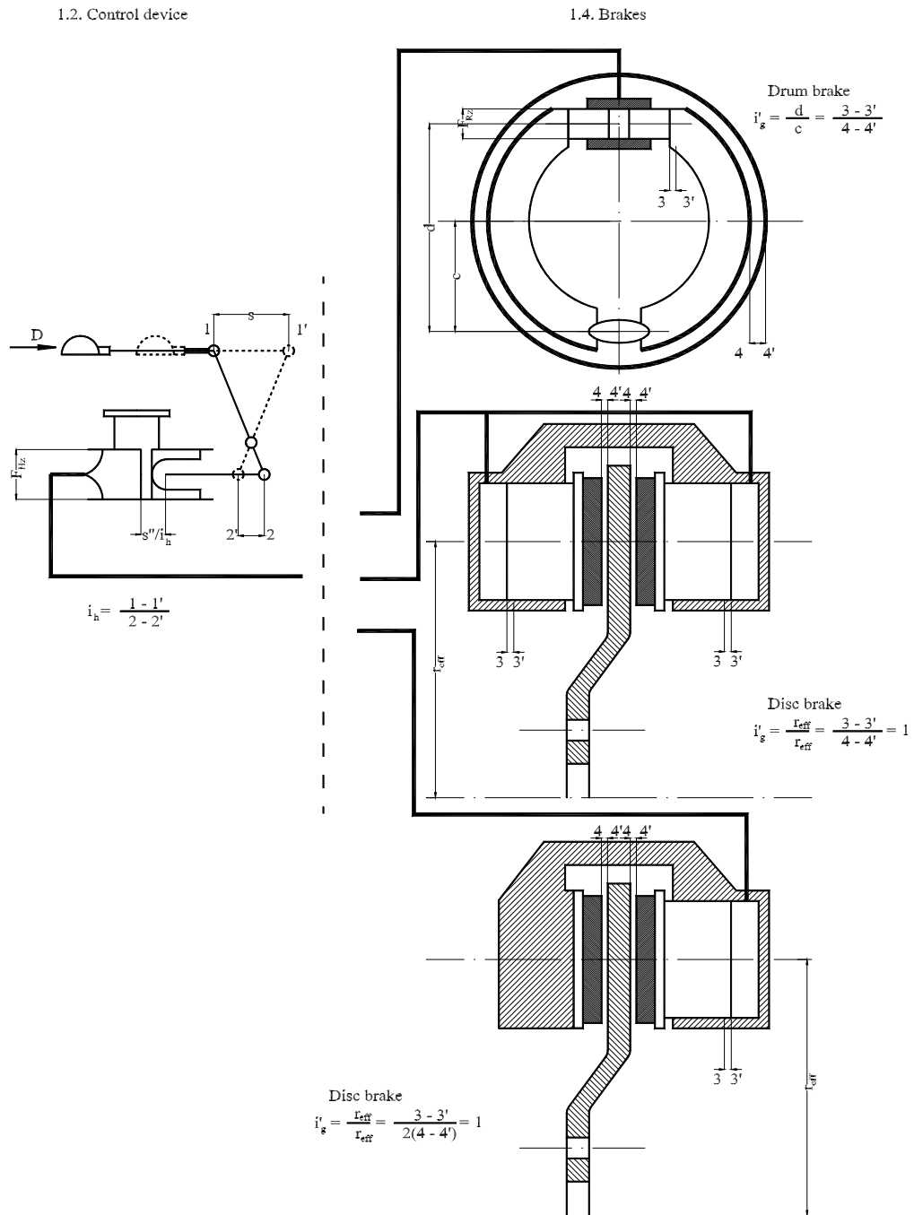
Figure 8: HYDRAULIC TRANSMISSION BRAKING SYSTEM (See paragraph 2.4. of this annex)
