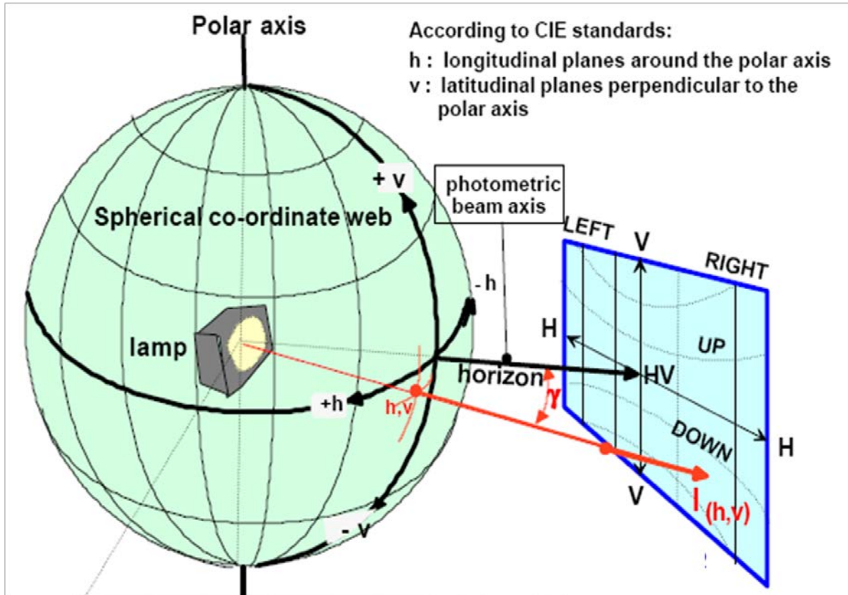
Figure A Spherical coordinate measuring system
