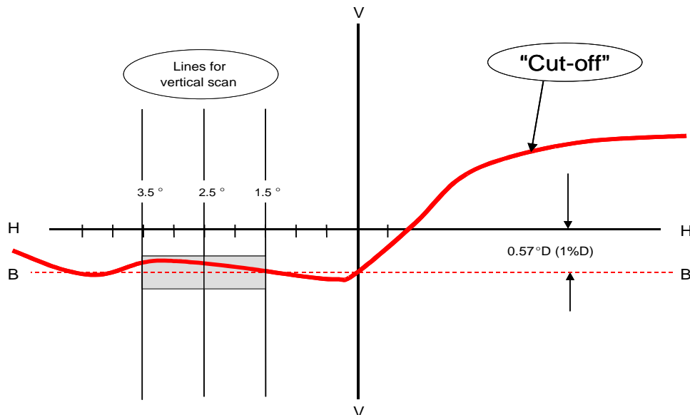
Figure 1 Measurement of "cut-off" quality
