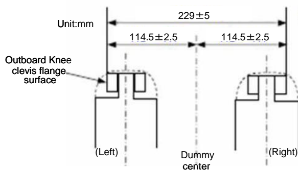
The initial knee distance of Hybrid III fifth percentile female
