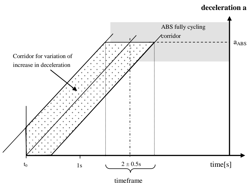
Deceleration corridor for determination of F_{ABS} and a_{ABS}
