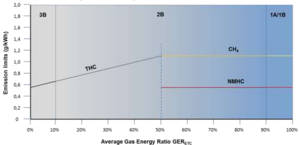
Figure 1 Illustration of the HC limits in the case of a dual-fuel engine operating in dual-fuel mode during the ETC cycle (natural gas dual-fuel engines)
