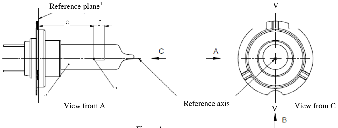
Figure 1 Main drawing
