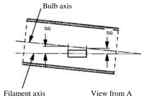
Figure 7 Bulb eccentricity
