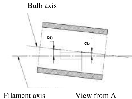
Figure 7 Bulb eccentricity
