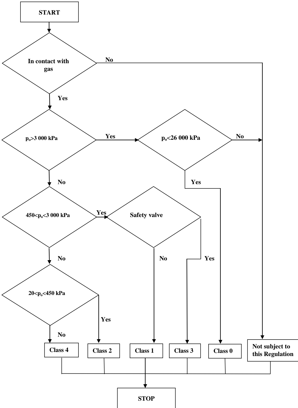
Figure 1-1 Flow scheme for CNG components classification
