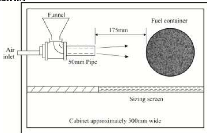
Figure H.2 Gravel impact test
