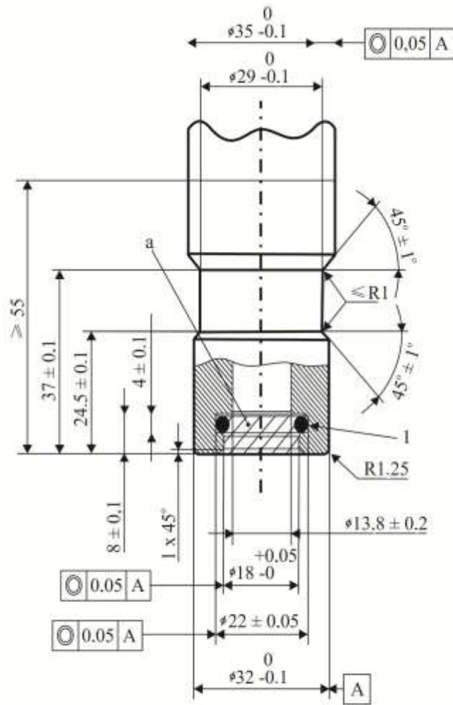
Figure 2 20 MPa Filling unit Size 2 (receptacle) for M 2 , M 3 , N 2 and N 3 vehicles Dimensions in millimetres
