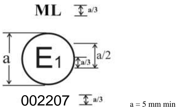
Figure 4 Marking for a manoeuvring lamps
