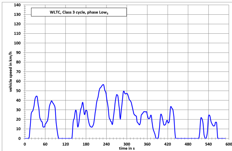
WLTC, Class 3 cycle, phase Low 3
