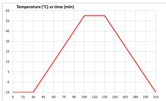
Figure C3/2 Temperature conditioning cycle
