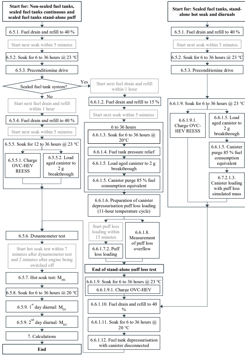
Figure C3/4 Test procedure flow charts
