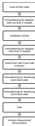
Figure C5.App1/1 Overview of demonstration test
