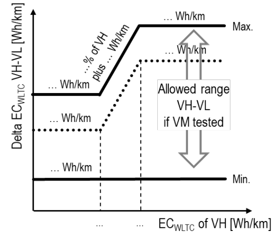
Figure A8/4a Interpolation range for EVs with vehicle M
