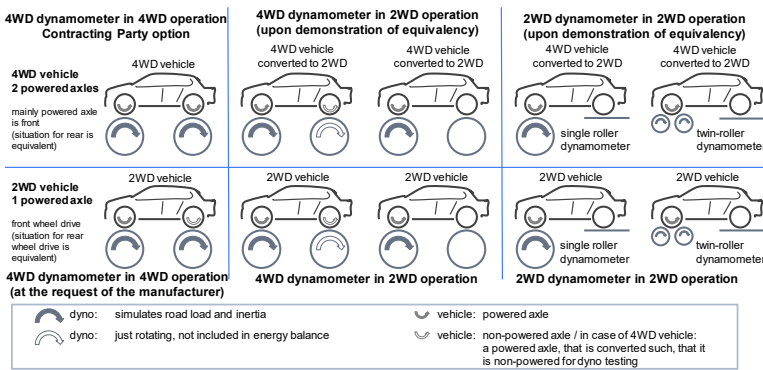
Figure A6/5a[xxx] Possible test configurations on 2WD and 4WD dynamometers
