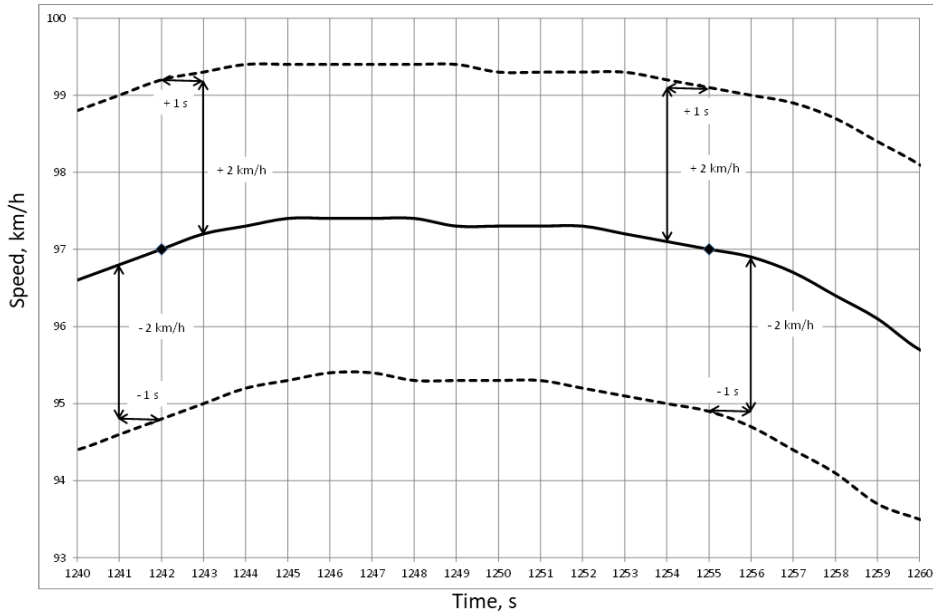
Figure A6/6 Speed trace tolerances
