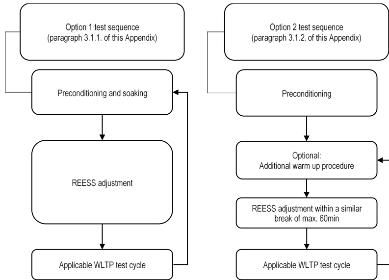
OVC-HEV and OVC-FCHV test sequences
