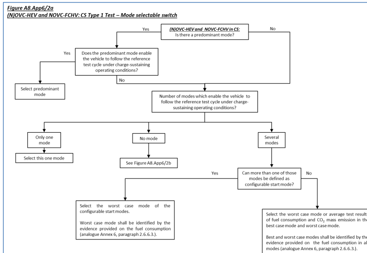
Figure A8.App6/2a and Figure A8.App6/2b Selection of a driver-selectable mode for OVC-HEVs, NOVC-HEVs, NOVC-FCHVs and NOVC-FCHVs under charge-sustaining operating condition
