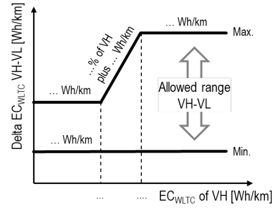
Figure A8/3a Interpolation range between vehicle H and vehicle L applied to EVs
