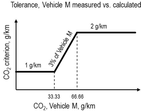
Figure A8/6 Linearity criterion for vehicle M
