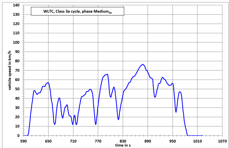
WLTC, Class 3a cycle, phase Medium 3a
