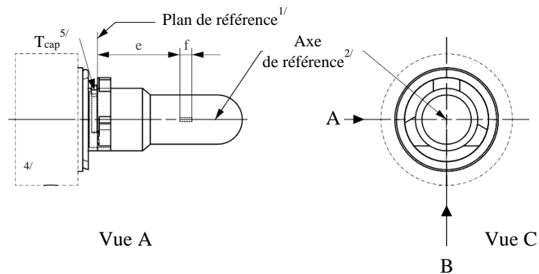
Figure 1 : Dessin principal
