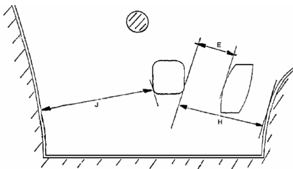
Figure 1b Two pedals – Automatic transmission with footrest
