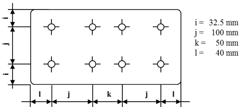
Measuring points for plate size 330 x 165 mm
