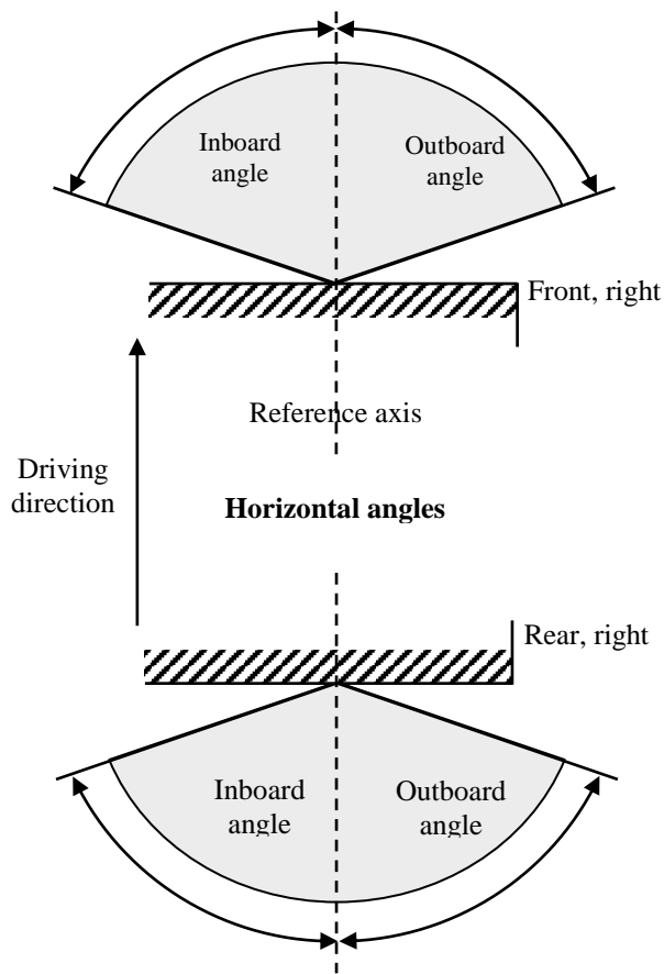
Figures A2-I: Light-distribution in space, horizontal and vertical
