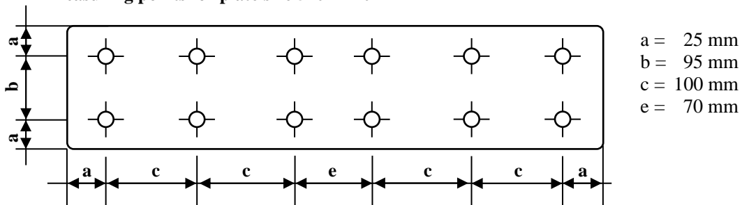
Measuring points for plate size 520 x 120 mm
