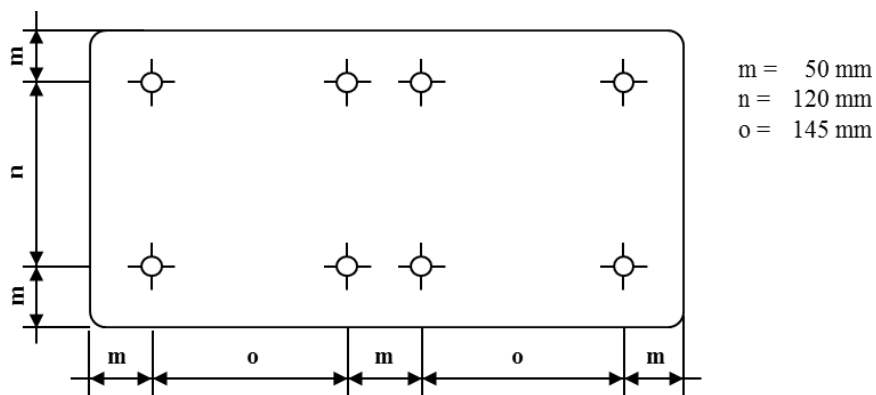
Measuring points for plate size 440 x 220 mm
