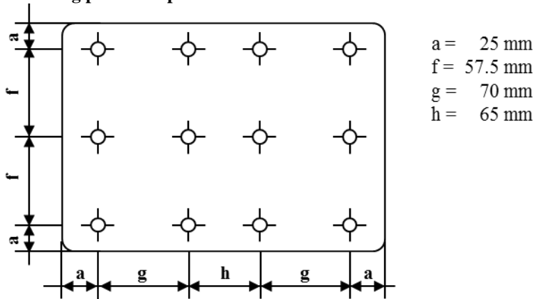
Measuring points for plate size 255 x 165 mm
