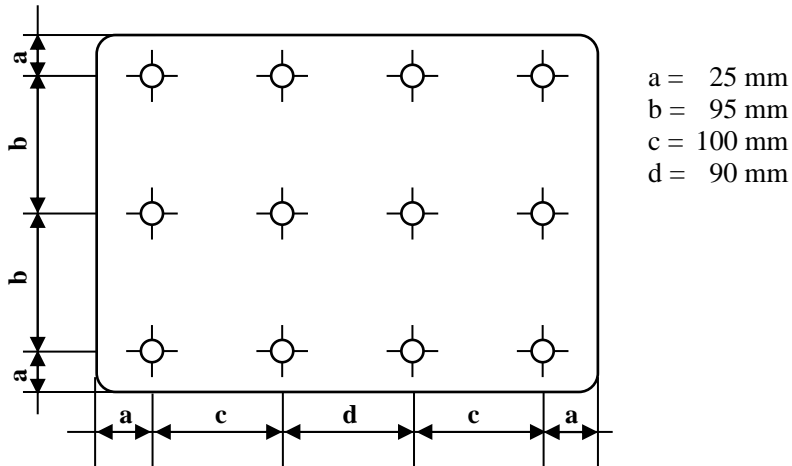
Measuring points for plate size 340 x 240 mm
