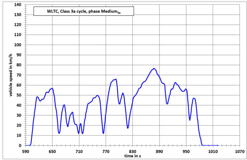
WLTC, Class 3a cycle, phase Medium 3a
