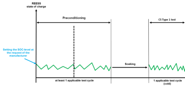
Figure A8.App1/2 OVC-HEVs, charge-sustaining Type 1 test
