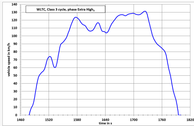
Figure A1/12 WLTC, Class 3 cycle, phase Extra High 3
