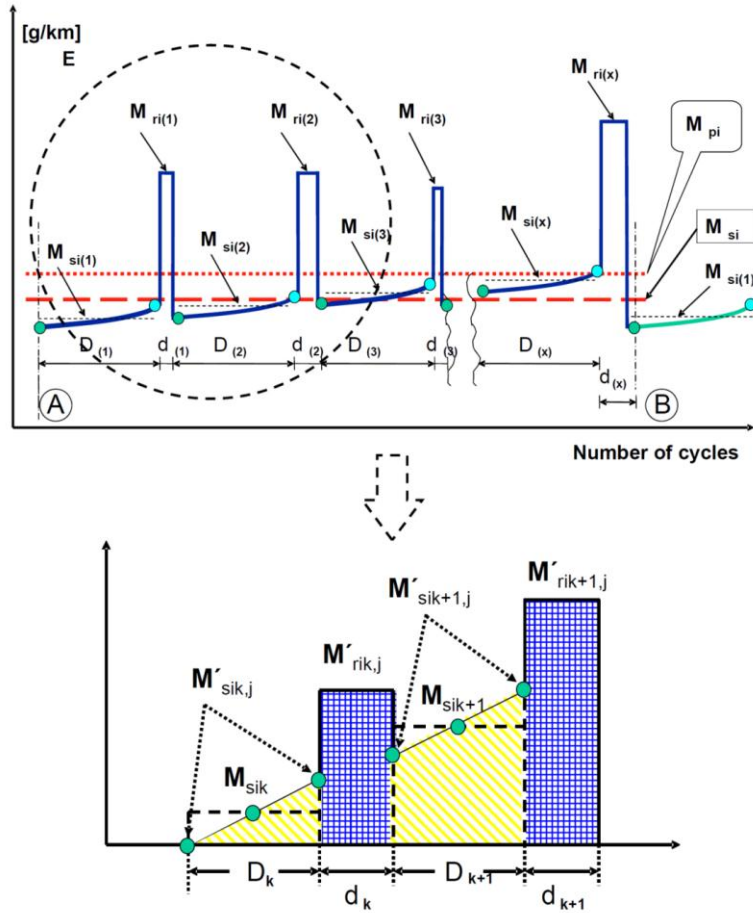
Figure A6.App1/2 Parameters measured during emissions test during and between cycles where regeneration occurs (schematic example)
