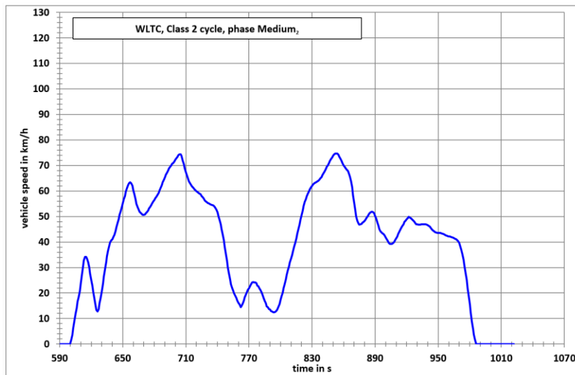
WLTC, Class 2 cycle, phase Medium 2
