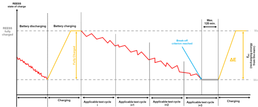
Figure A8.App1/6 Consecutive cycles test sequence PEV
