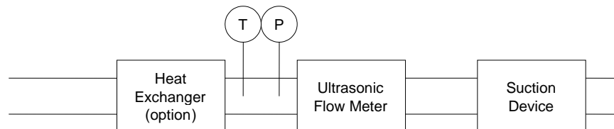
Schematic of an ultrasonic flow meter (UFM)
