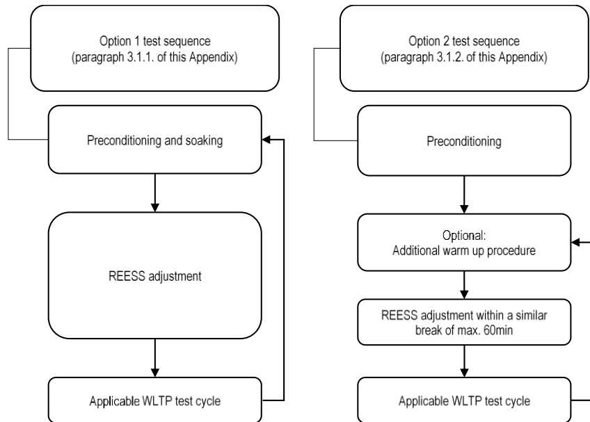
Figure A8.App2/1 OVC-HEV test sequences
