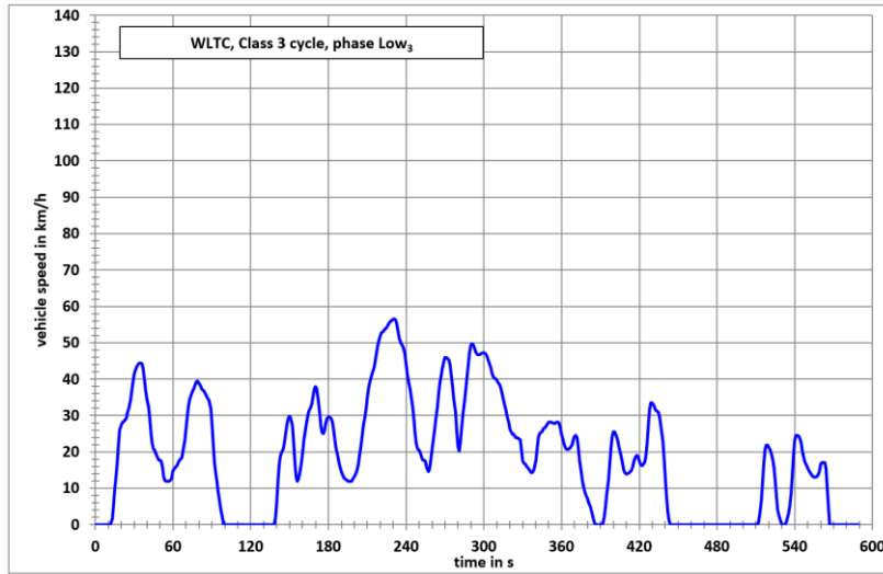
WLTC, Class 3 cycle, phase Low 3
