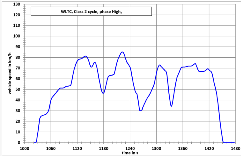
Figure A1/5 WLTC, Class 2 cycle, phase High 2
