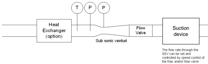
Schematic of a subsonic venturi tube (SSV)
