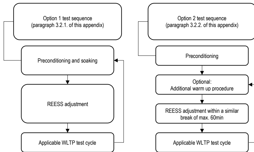
Figure A8.App2/2 NOVC-HEV and NOVC-FCHV test sequences
