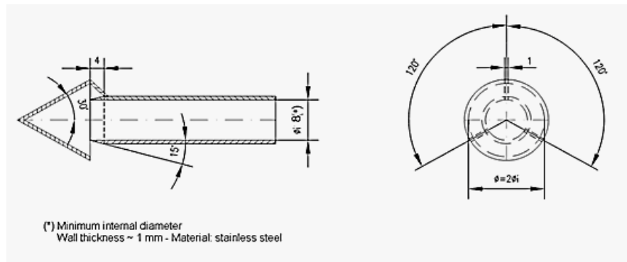
Figure A5/11 Alternative particulate sampling probe configuration
