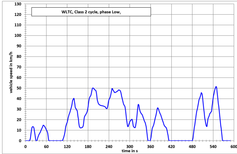
WLTC, Class 2 cycle, phase Low 2
