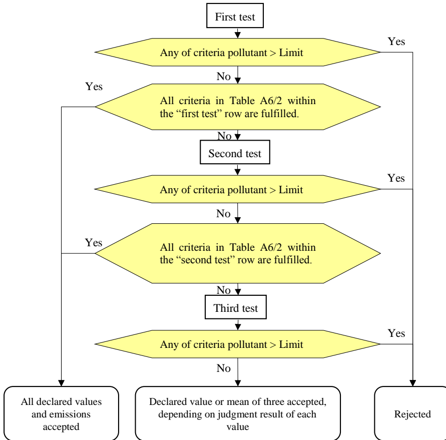
Flowchart for the number of Type 1 tests
