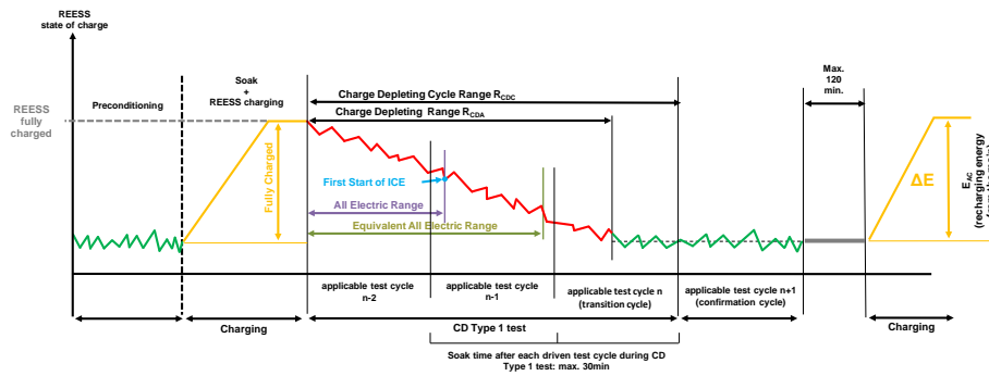
Figure A8.App1/1 OVC-HEVs, charge-depleting Type 1 test
