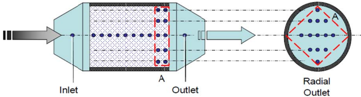
Figure 2 Example of temperature sensors location for DPF
